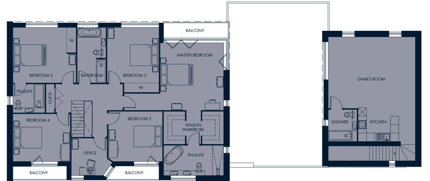
FIRST FLOOR
