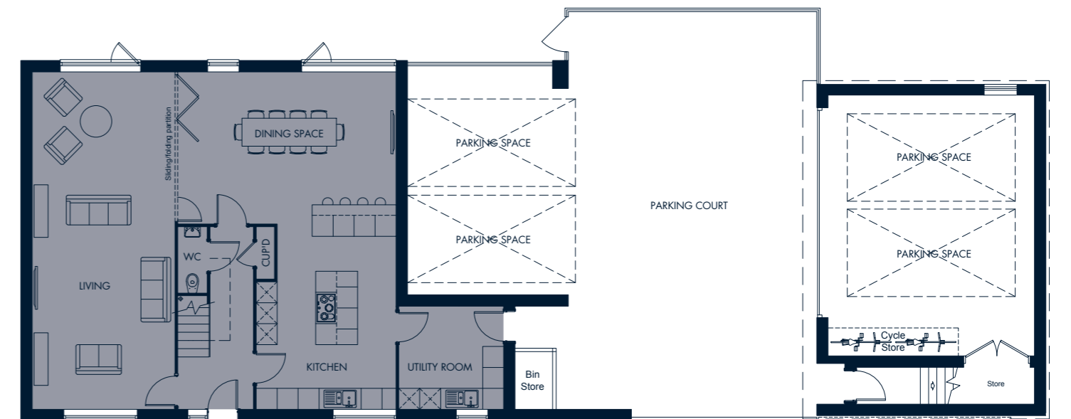
GROUND FLOOR
