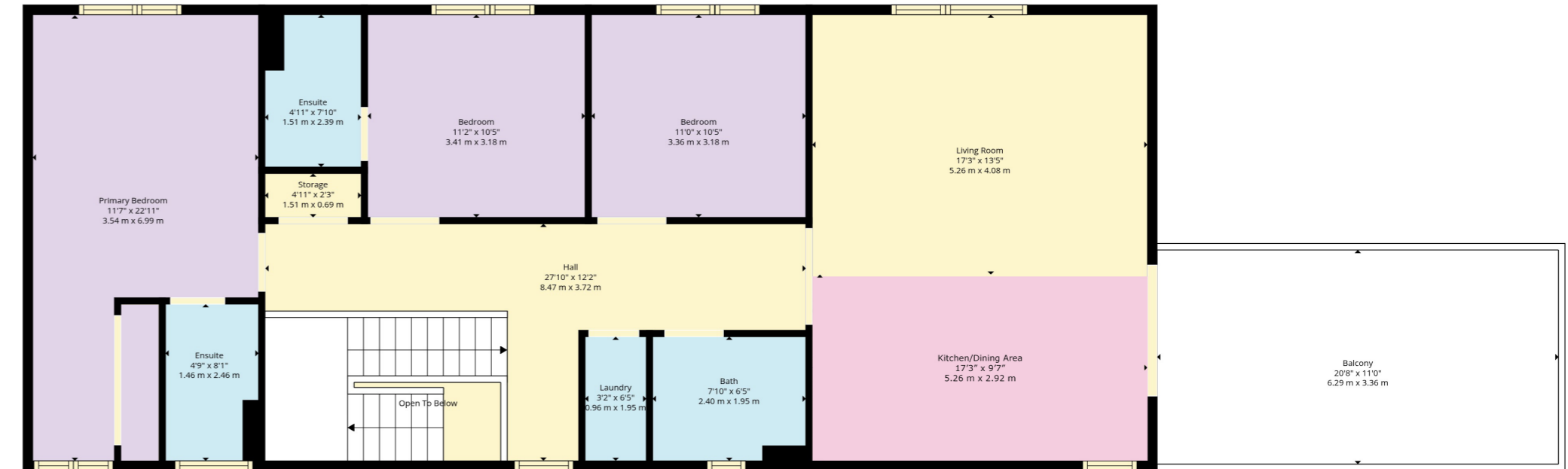
Floor 2
