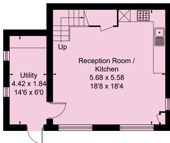
Outbuilding 1 - Ground Floor
