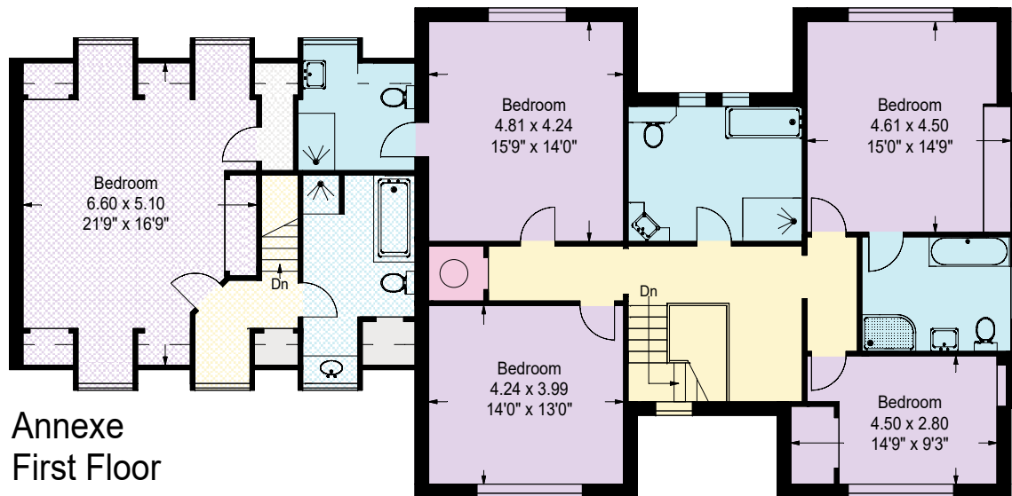
First Floor
