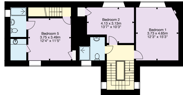
First Floor
