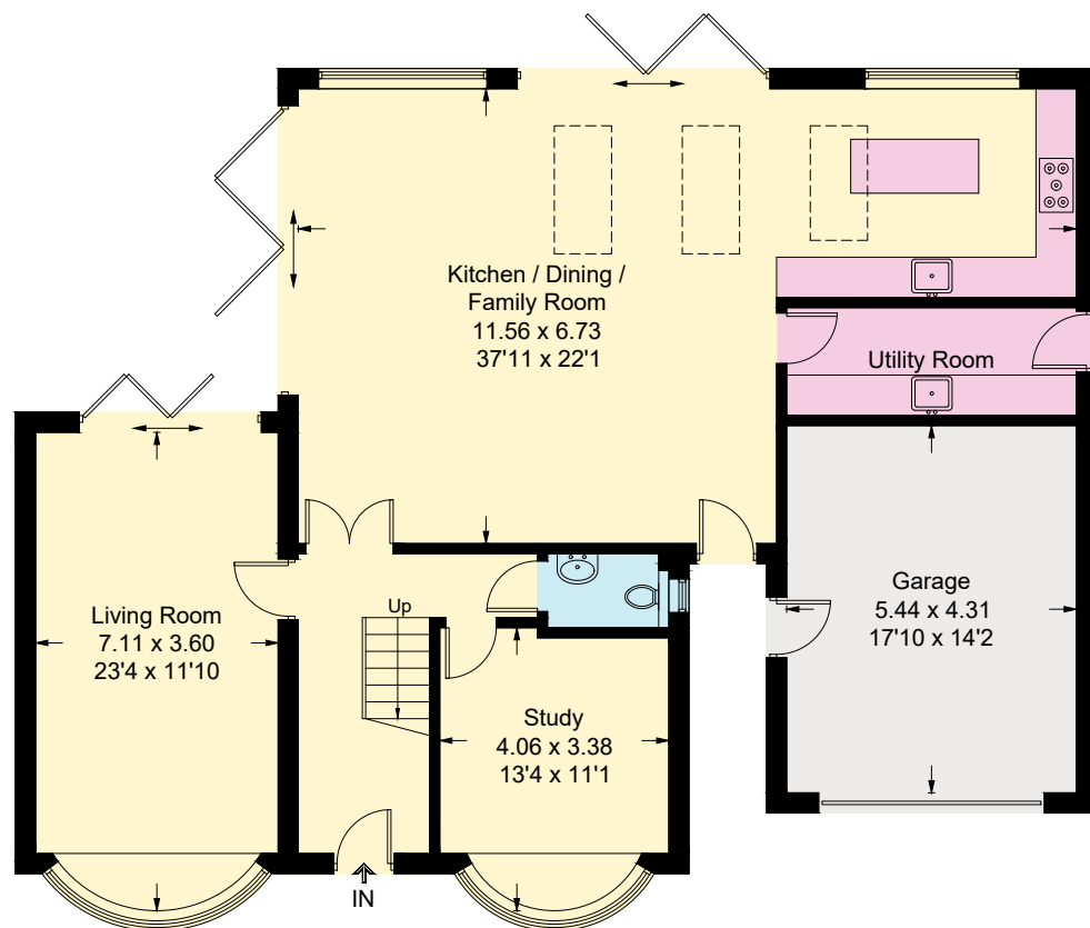
Ground Floor
