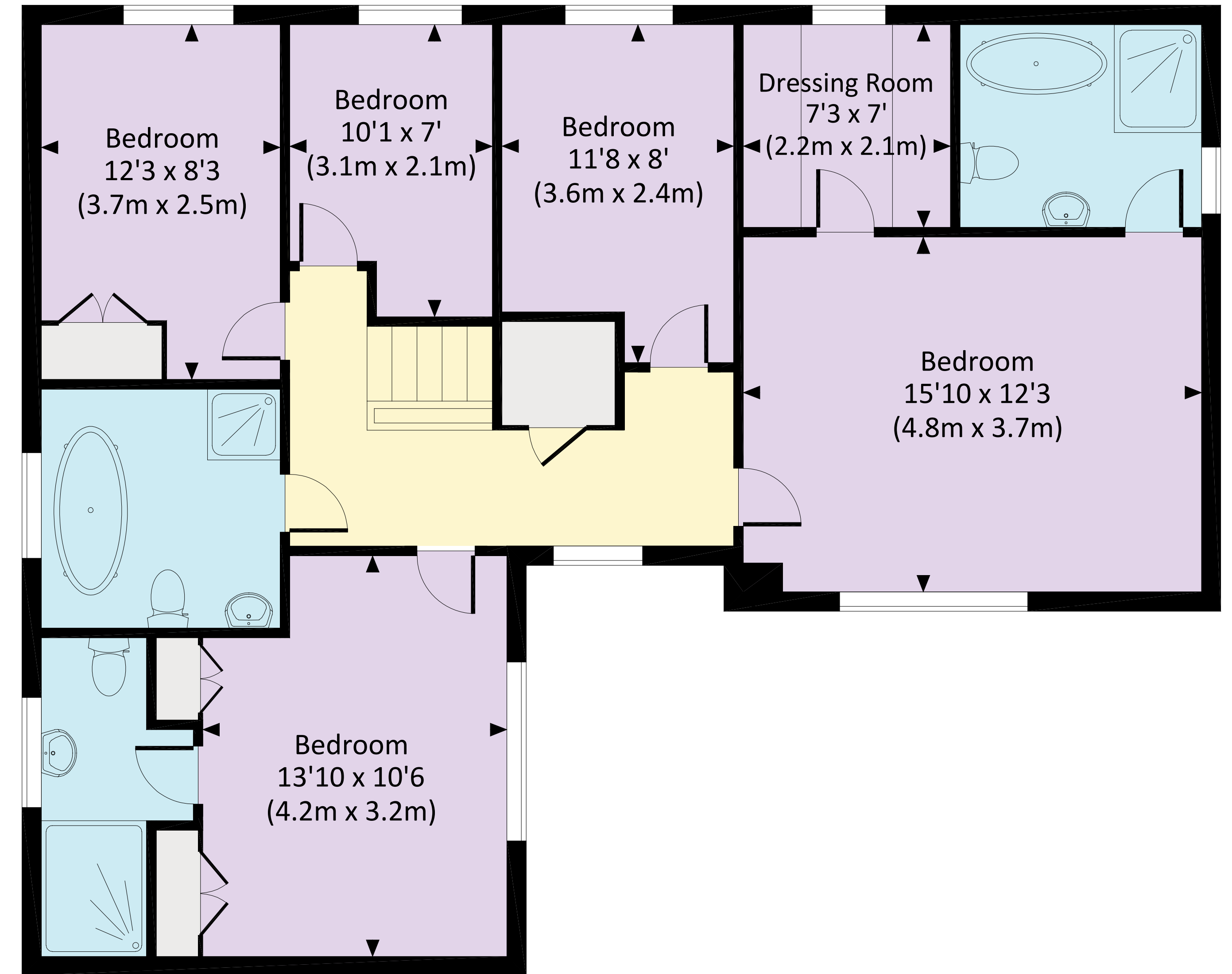
FIRST FLOOR
