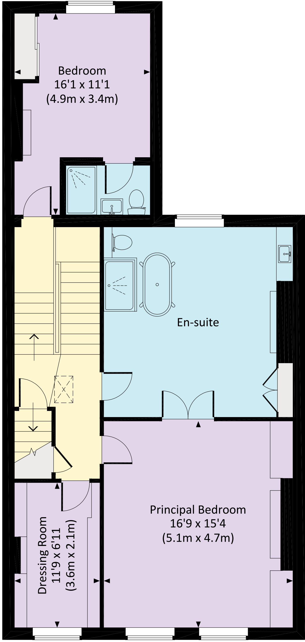
FIRST FLOOR
