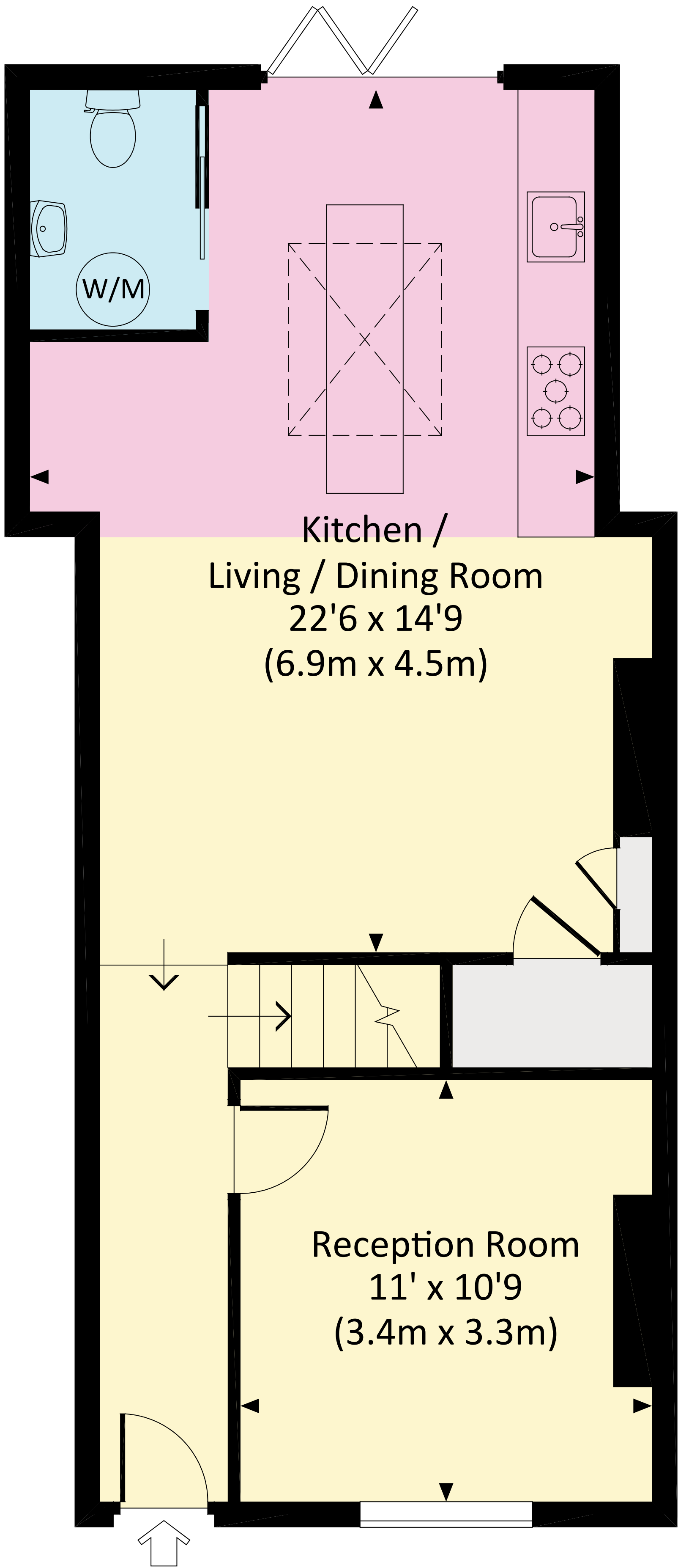
GROUND FLOOR
