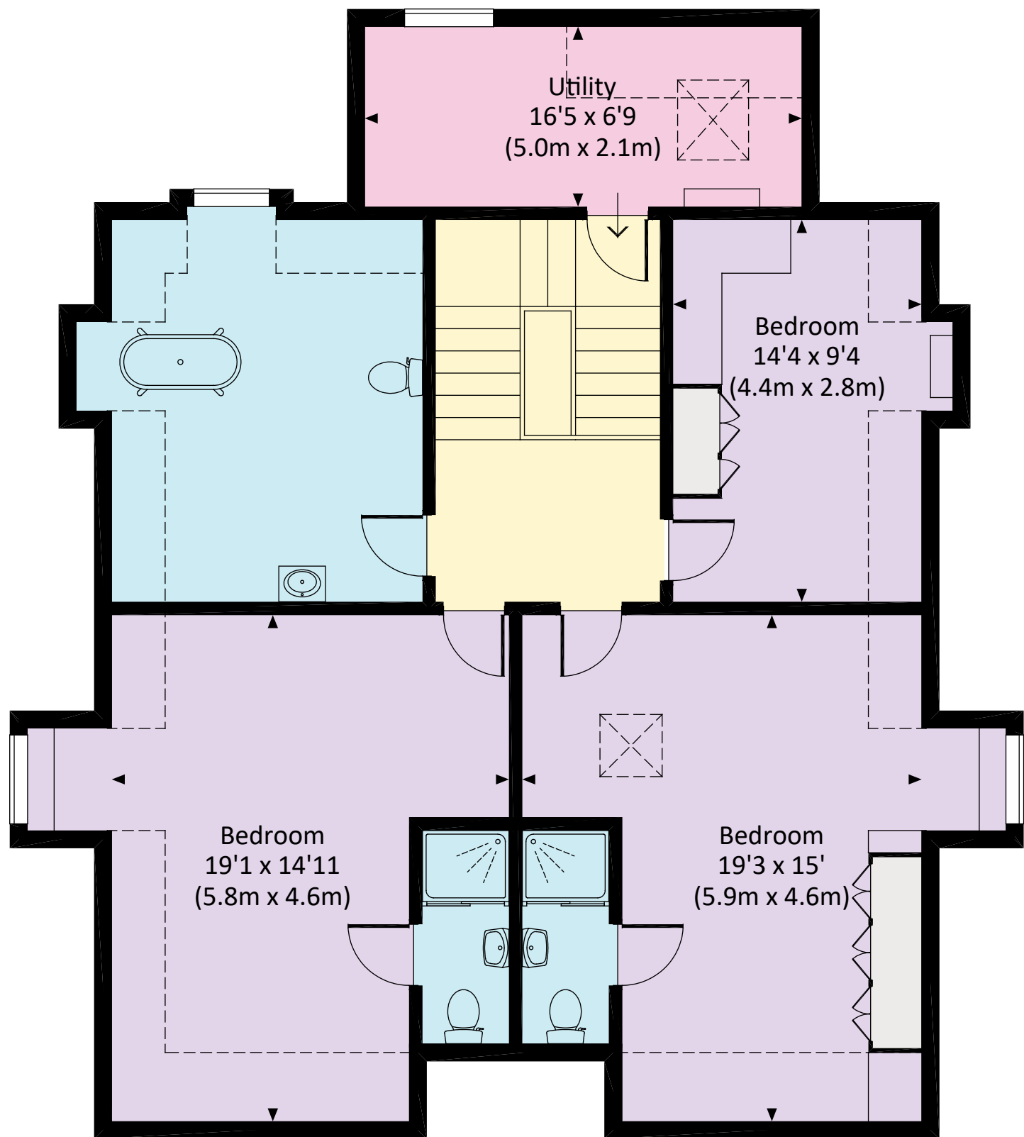
SECOND FLOOR
