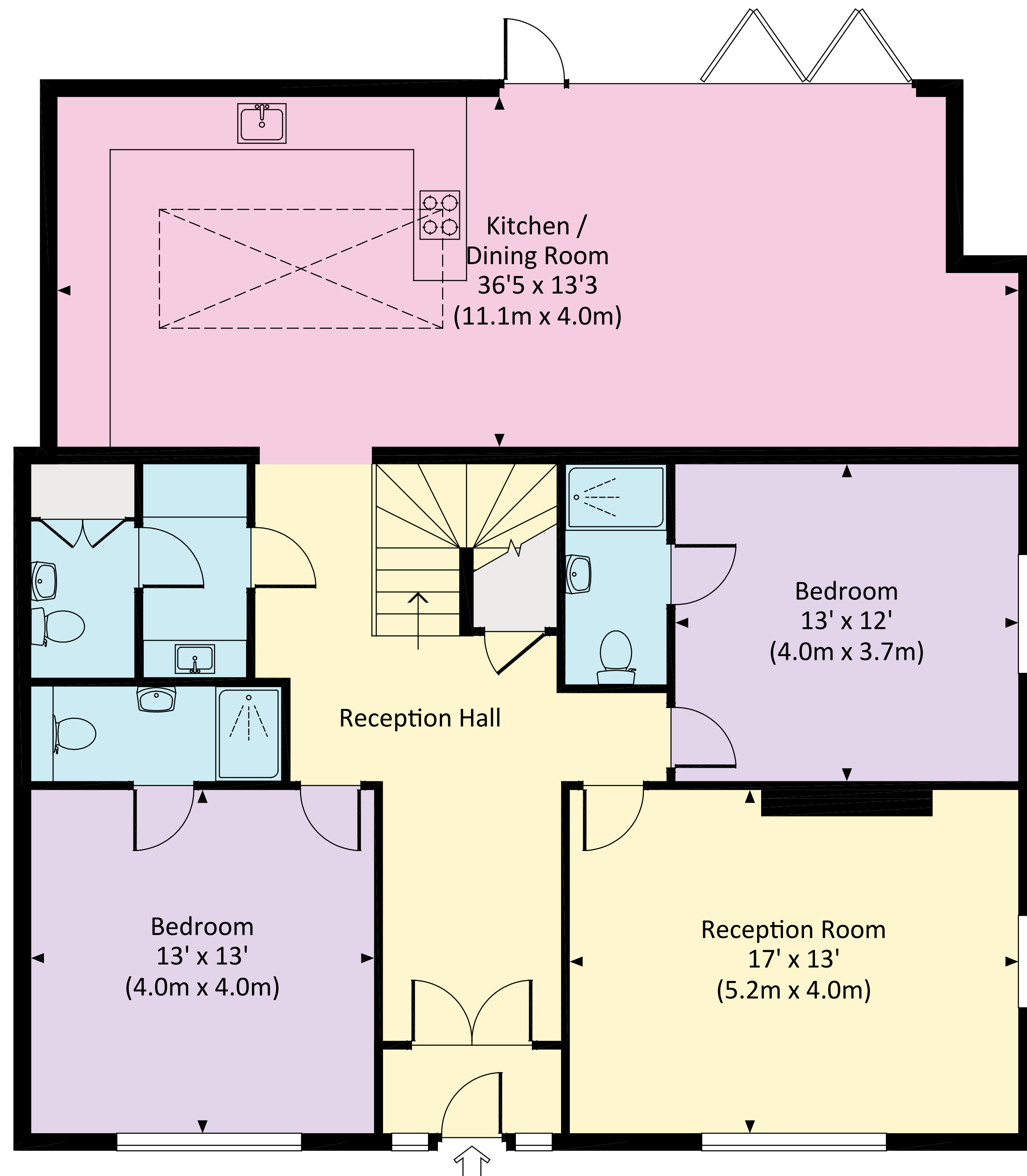
GROUND FLOOR
