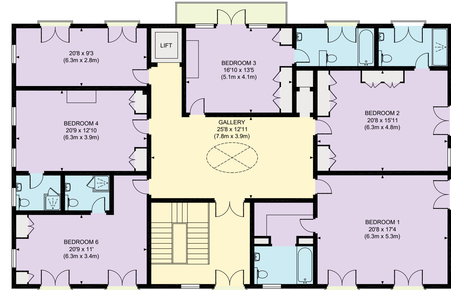
FIRST FLOOR
