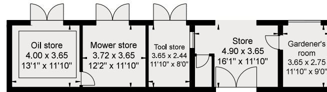
Outbuilding
