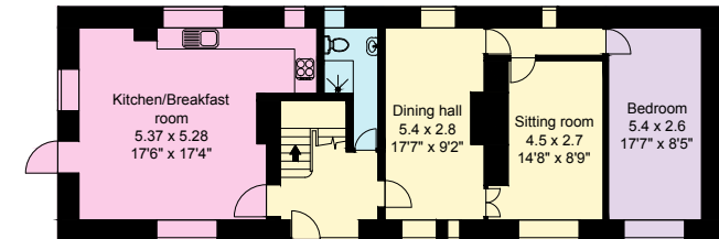
The Courtyard Ground Floor
