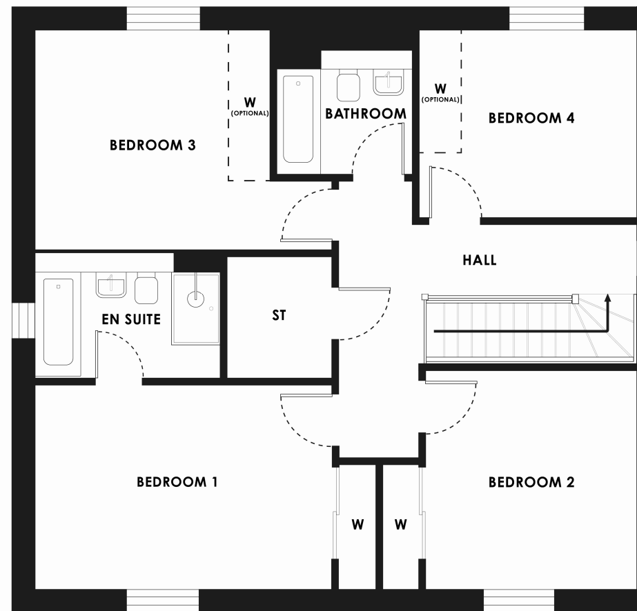
FIRST FLOOR
