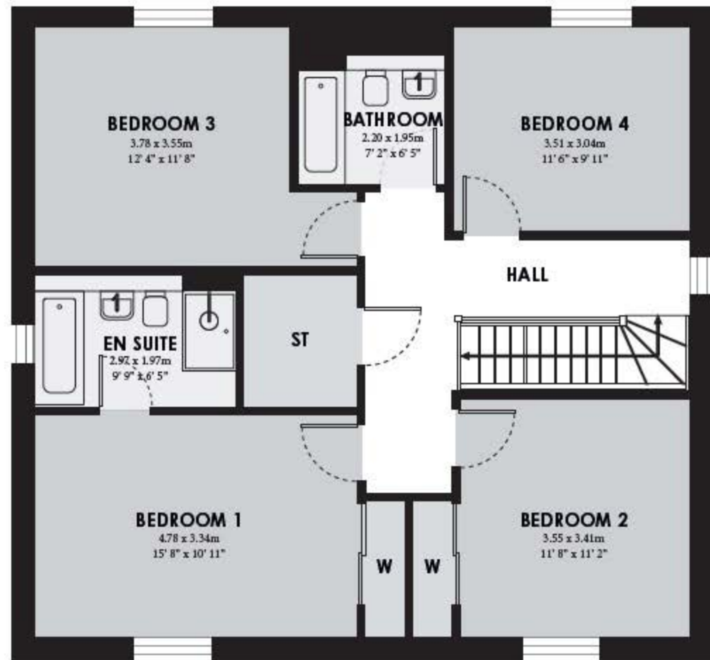
First Floor
