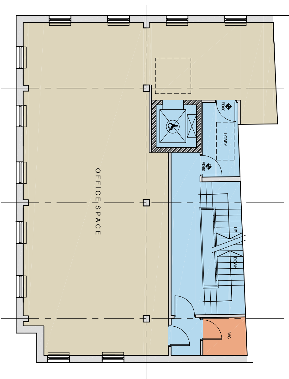
LEVEL 05 PLAN - 1:100
