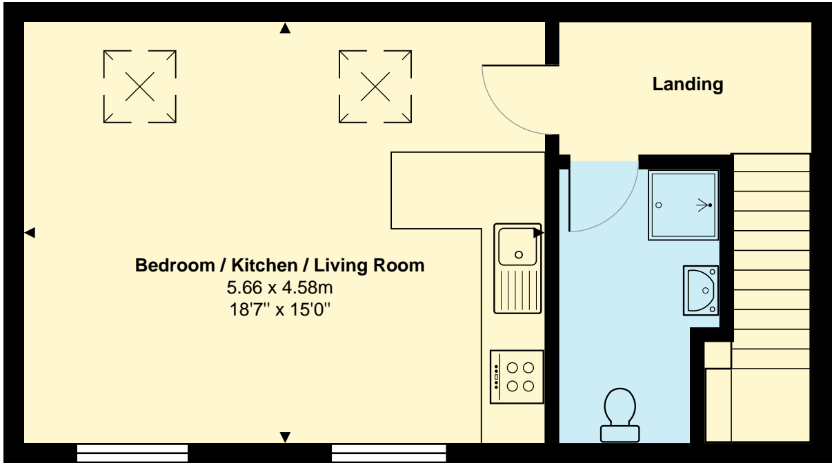
Area: 39.2 m 2 ... 422 ft 2 The Shippen First Floor
