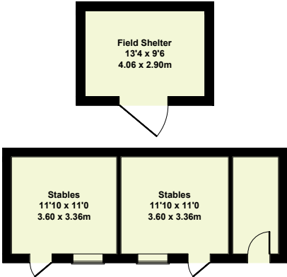
OUTBUILDINGS
