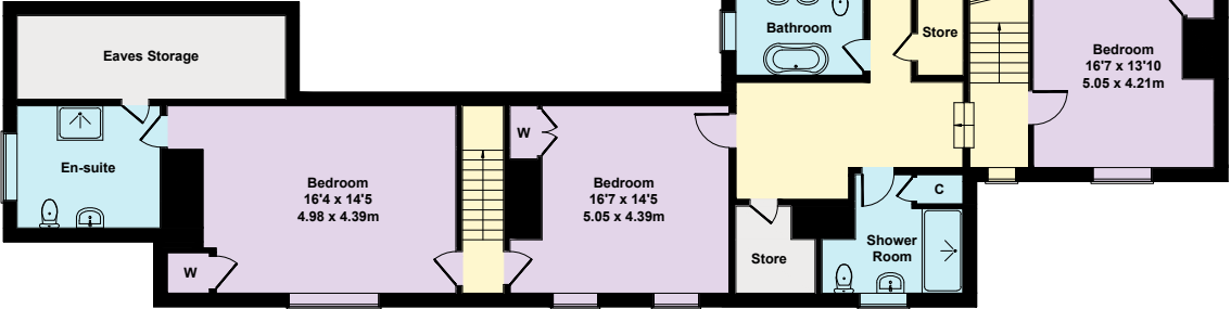
FIRST FLOOR
