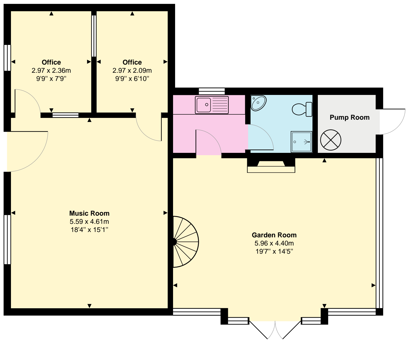
Studio Ground Floor Area: 79.2 m 2 ... 853 ft 2
