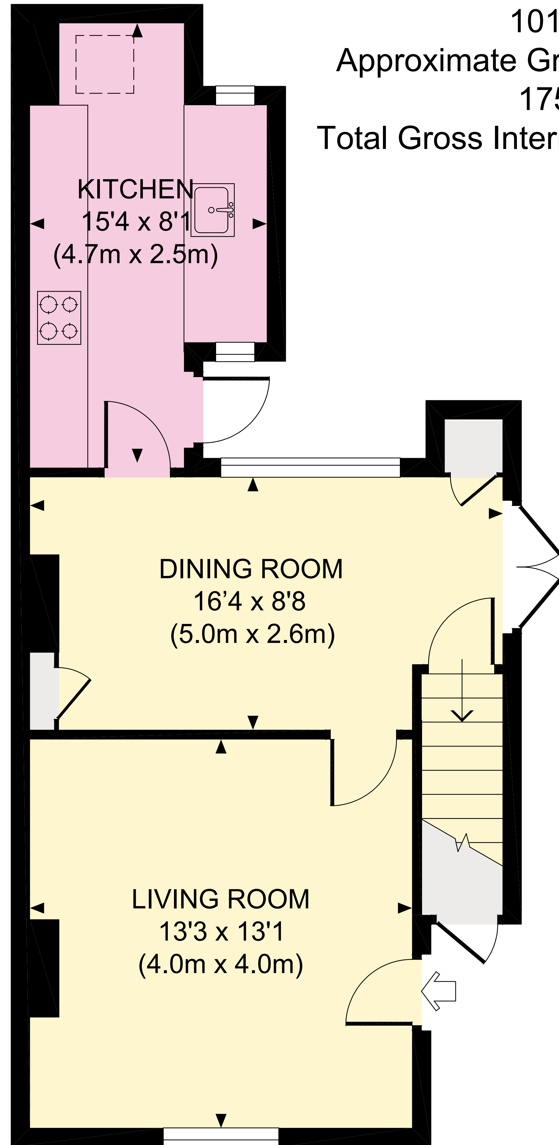
GROUND FLOOR
