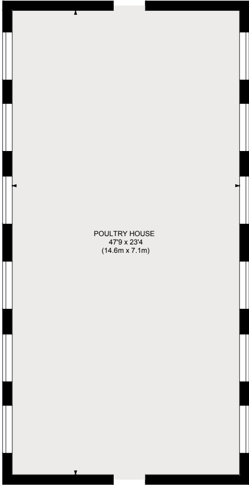
OUTBUILDING
