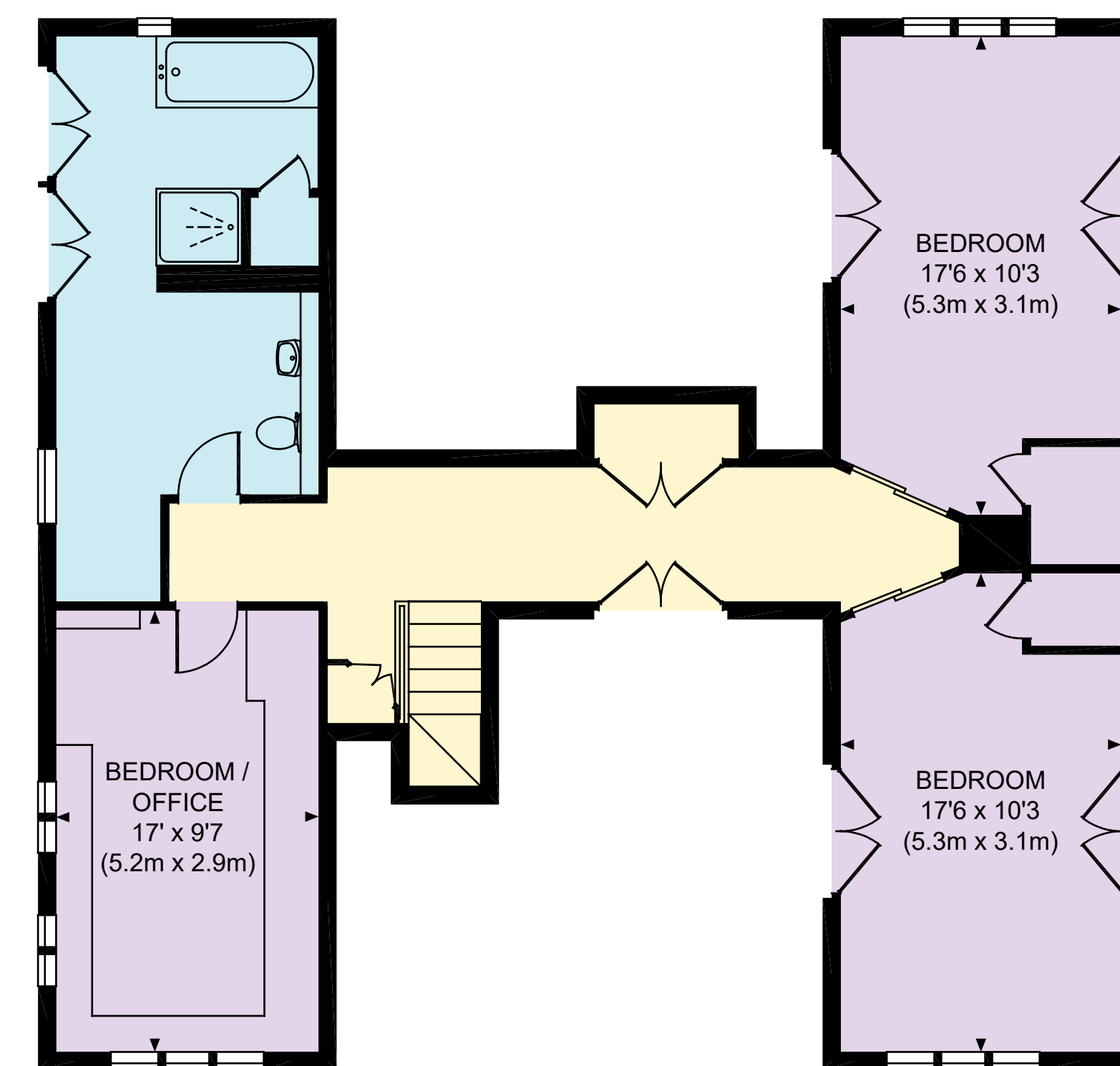
SECOND FLOOR
