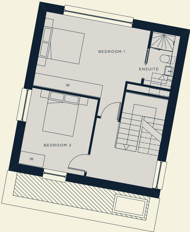
SECOND FLOOR
