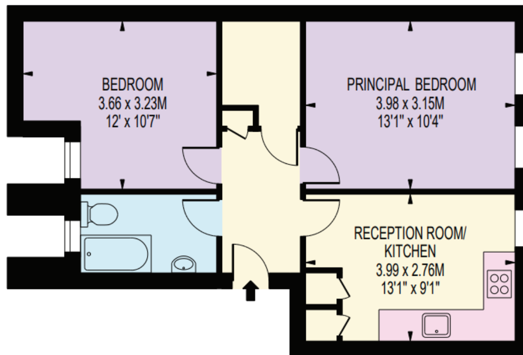
SECOND FLOOR
