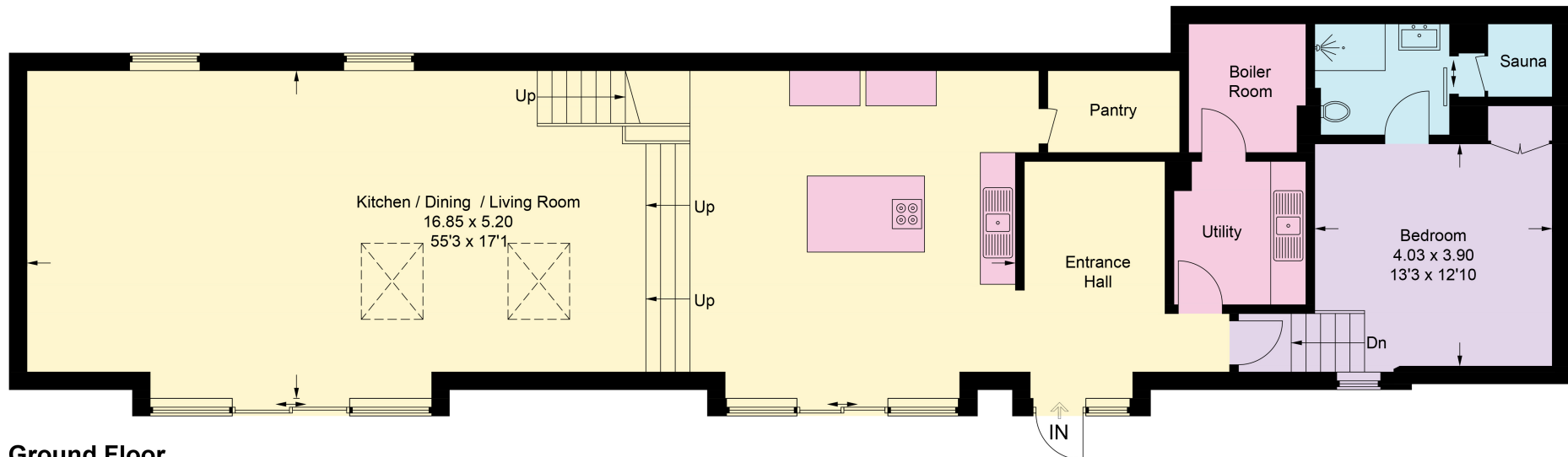
Ground Floor
