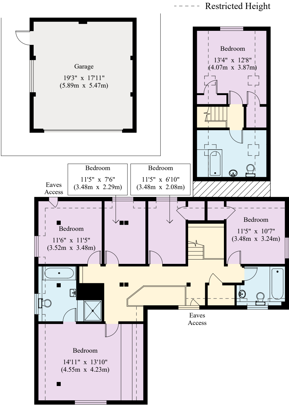
First Floor
