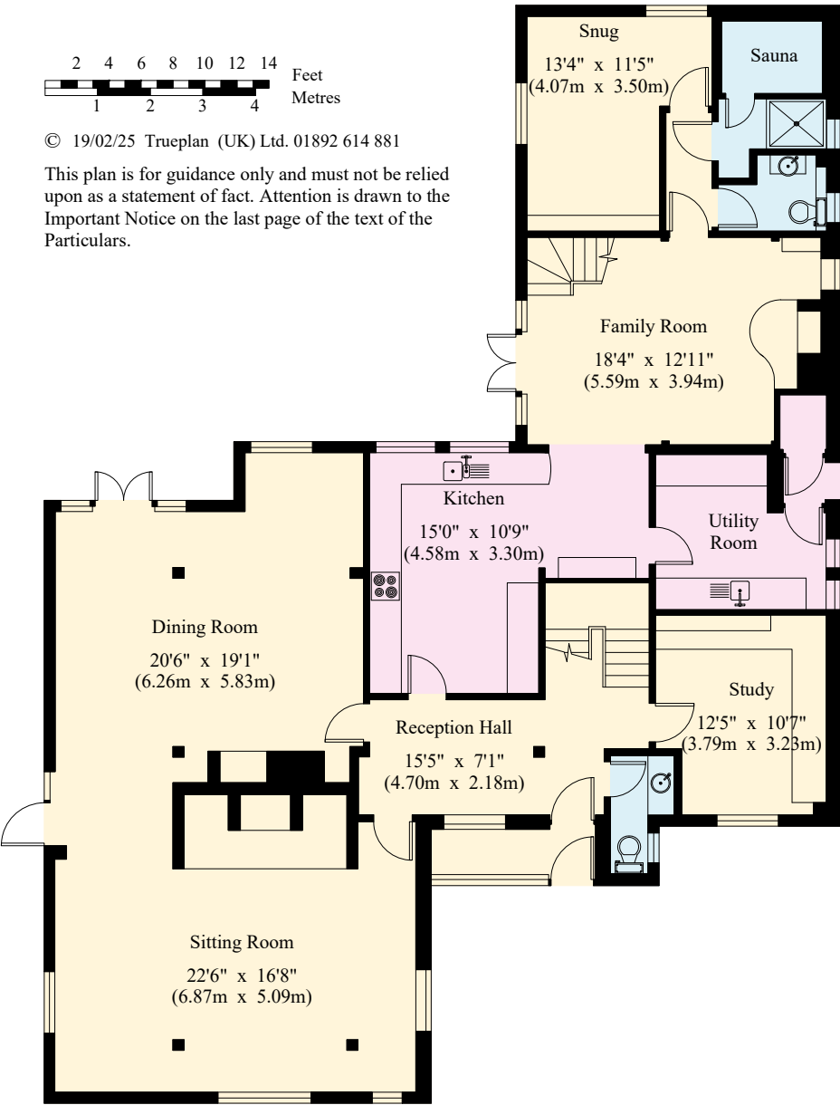
Ground Floor
