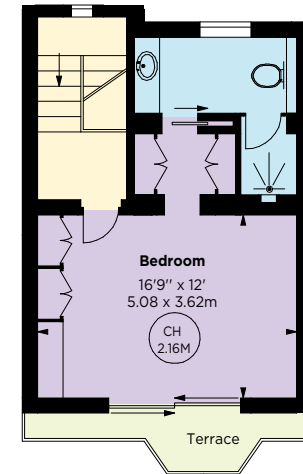
FOURTH FLOOR
