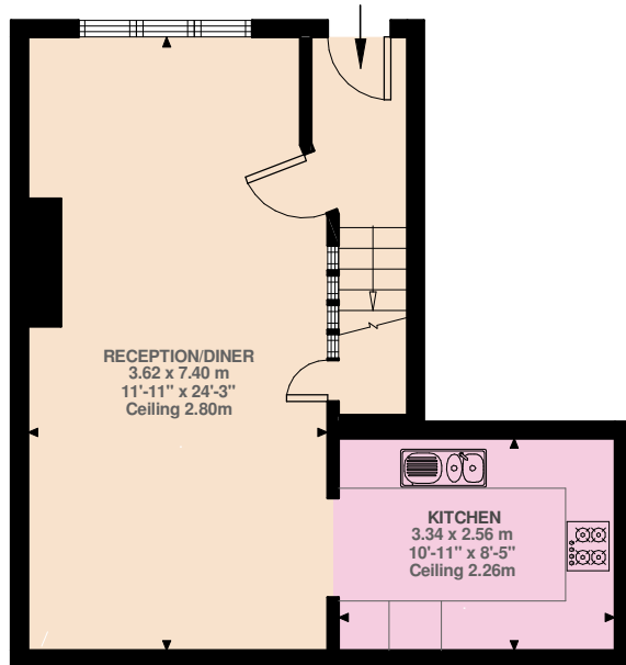
Ground Floor 434 ft 2
