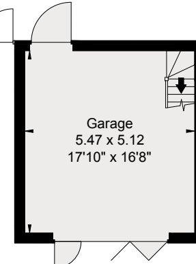
Outbuilding Ground floor
