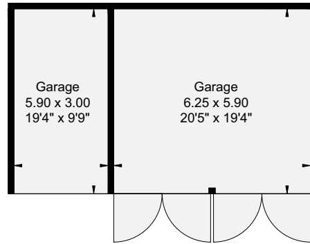
Proposed Outbuilding
