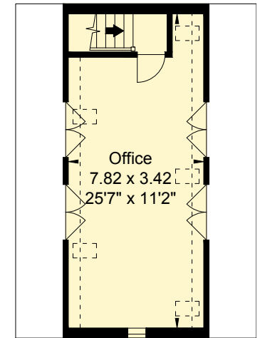
Outbuilding First Floor
