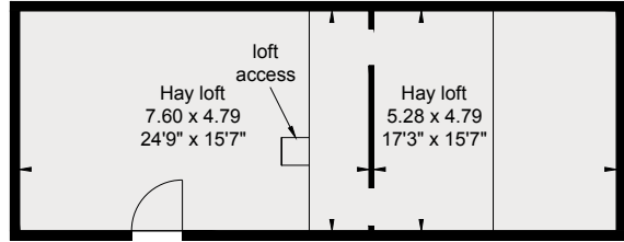
Outbuilding First Floor
