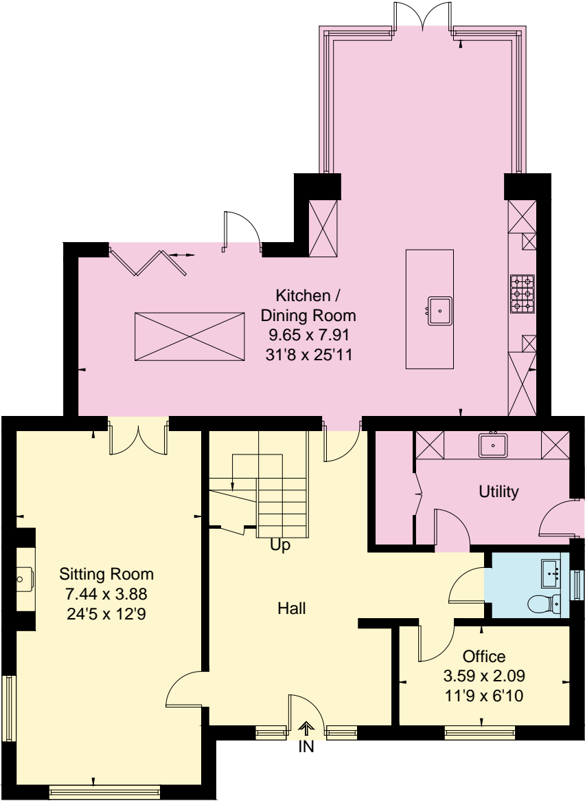
Ground Floor
