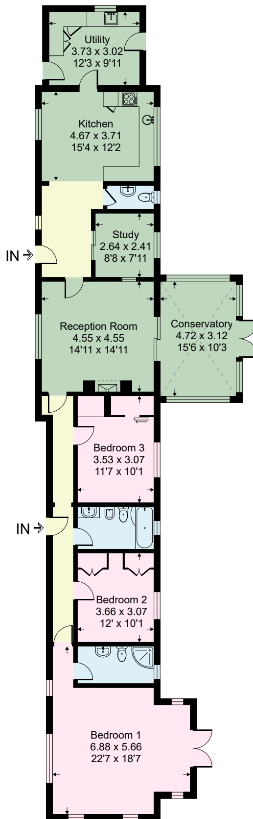
Ground Floor
