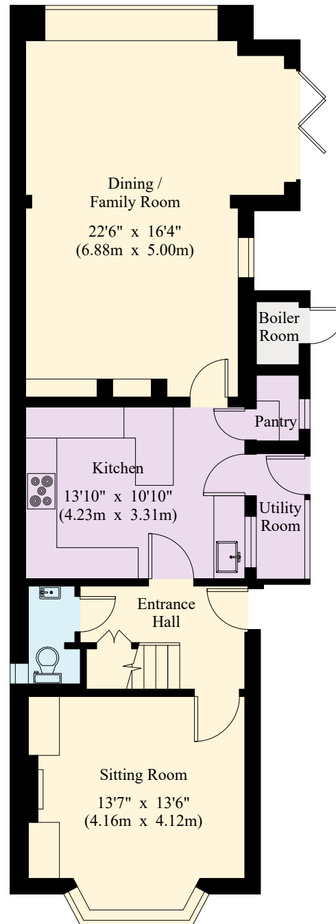
Ground Floor
