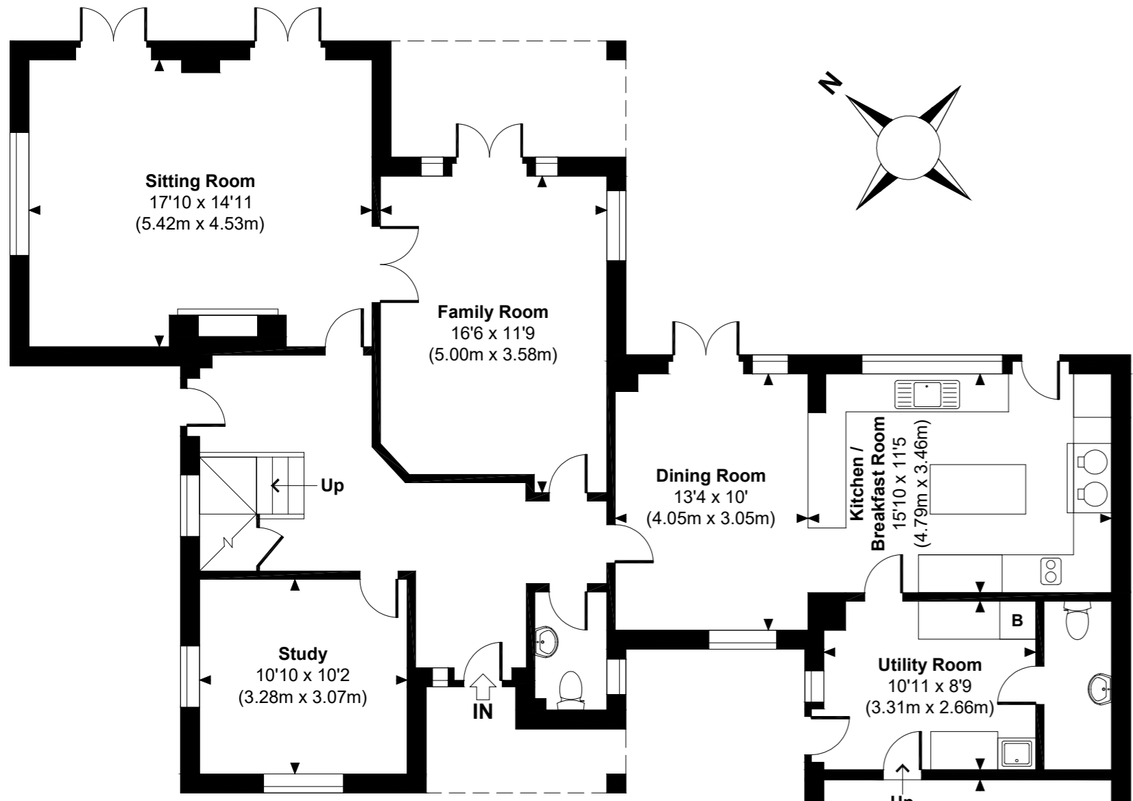
GROUND FLOOR
