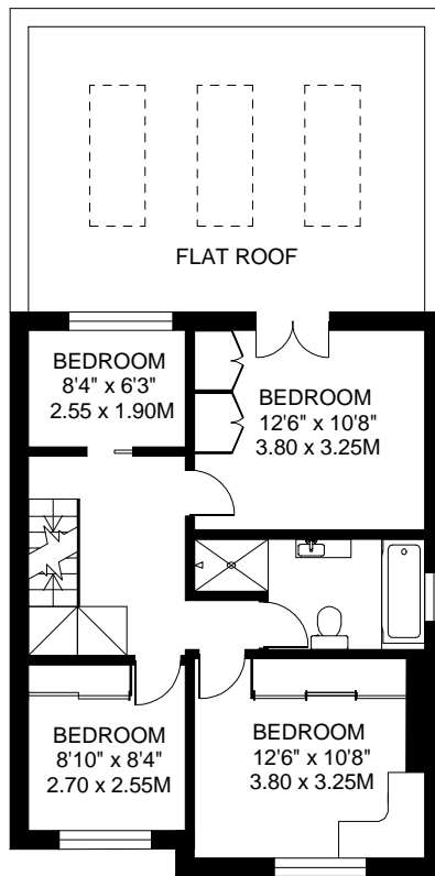
FIRST FLOOR 584 SQ.FT.
