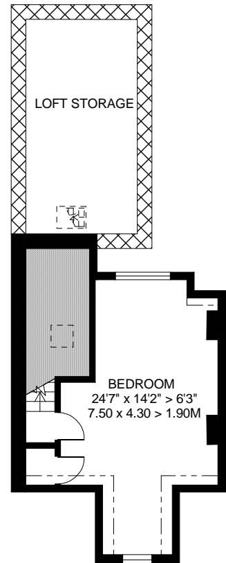
SECOND FLOOR 292 SQ.FT.
